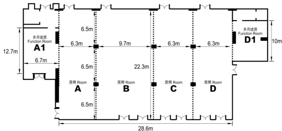
宴會廳 - 平面圖 (700平方米) Grand Ballroom - Floor Plan (700m 2 )
