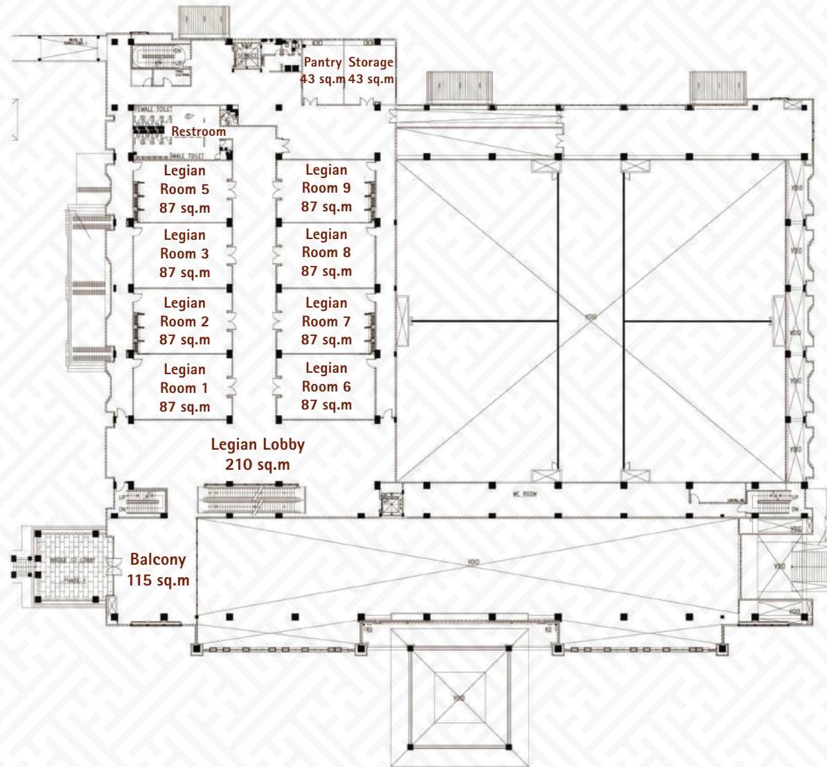
Mezzanine Floor
